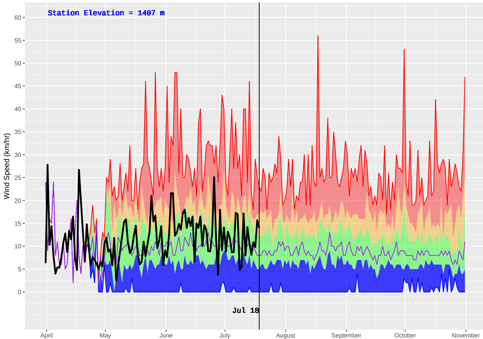
THYNNNE (279) : Historical (1977–2016) and Current (2018) Daily Wind Speed
