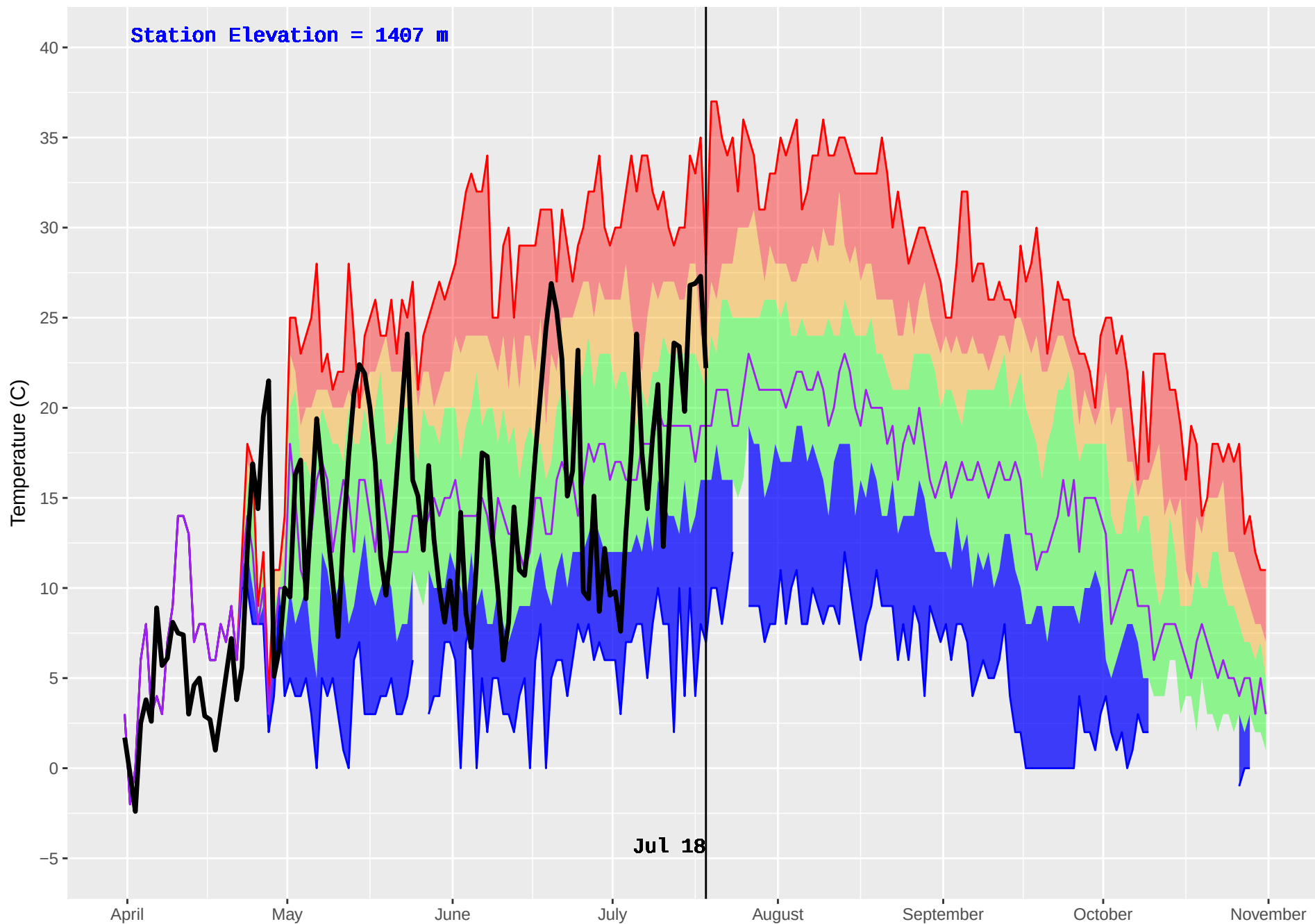
THYNNNE (279) : Historical (1977–2016) and Current (2018) Daily Temperature
