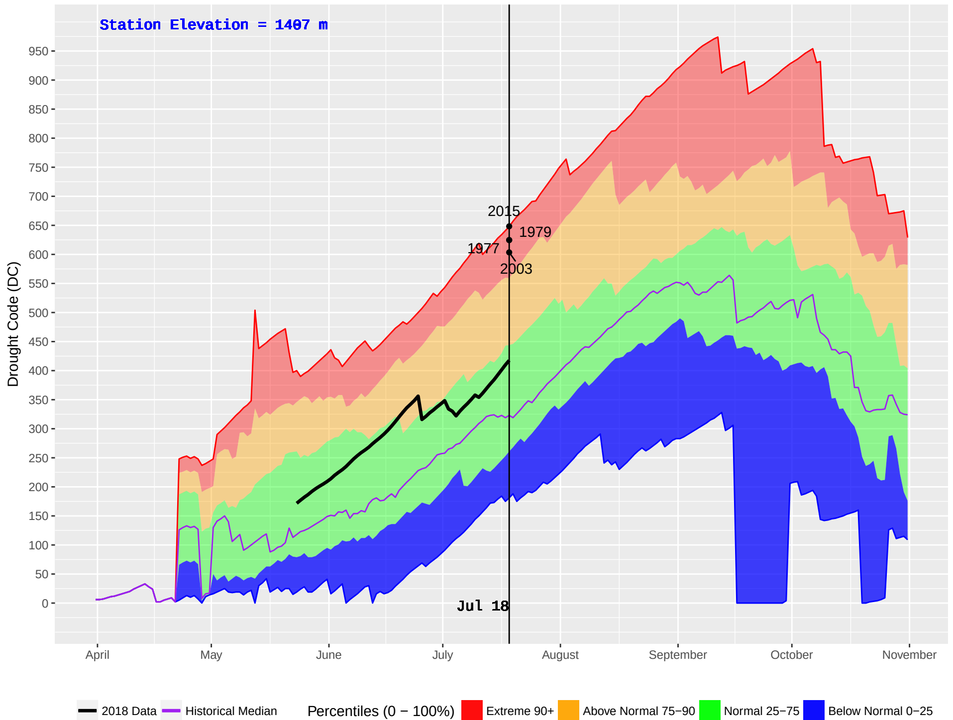
THYNNE (279) : Historical (1977–2016) and Current (2018) Daily Drought Code (DC)
