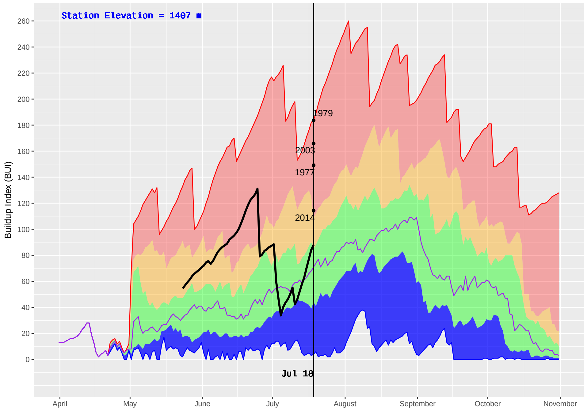
THYNNE (279) : Historical (1977–2016) and Current (2018) Daily Buildup Index (BUI)
